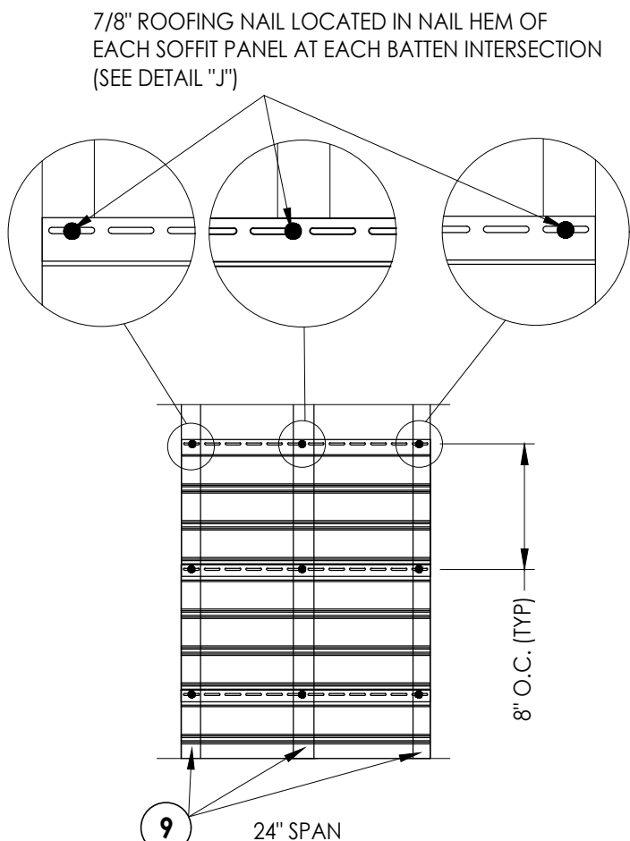
DETAIL "E"
