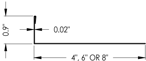
1 FASCIA Aluminum
