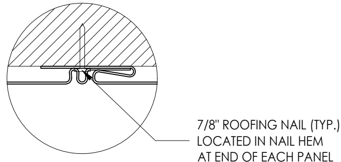
DETAIL "J"
