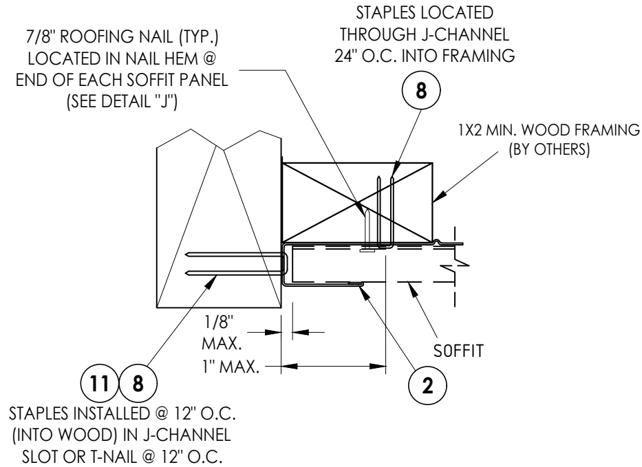
DETAIL "D" J-Channel Fascia
