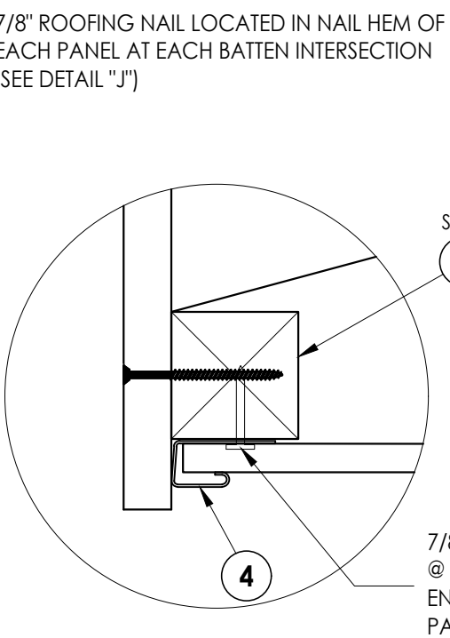
DETAIL "E"
